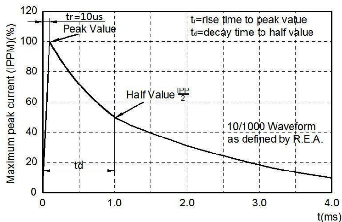
FIG3: Pulse Waveform
