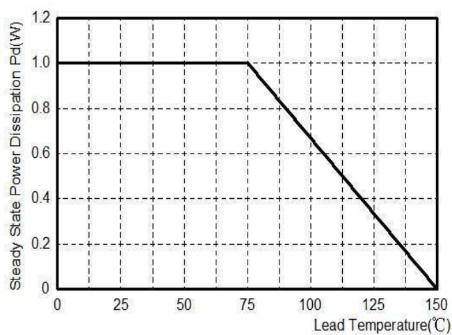
FIG5: Steady State Power Dissipation
